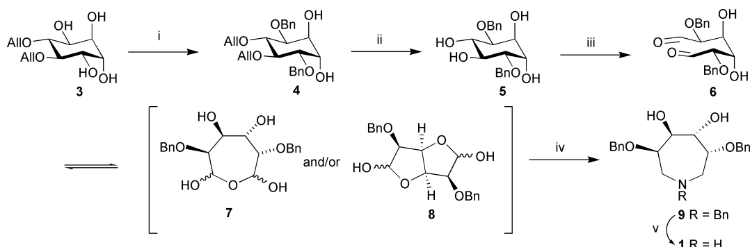
Scheme 1 Reagents, conditions and yields: i, (\text{Bu}_3\text{Sn})_2\text{O} , PhMe, 110 °C, 1.5 h, then BnBr, \text{Bu}_4\text{NBr} , PhMe, 110 °C, 2 h (53%); ii, Pd/C, TsOH, MeOH, 64 °C, 12 h (60%); iii, \text{NaIO}_4 , \text{H}_2\text{O} , MeCN, rt, 15 h, (86%); iv, \text{BnNH}_2 , \text{NaCNBH}_3 , AcOH, sieves, MeOH, -78 °C – rt, 10 h (60%); v, \text{Pd}(\text{OH})_2 , \text{NH}_4\text{OH} , MeOH, \text{H}_2 , rt, 12 h (57%).
